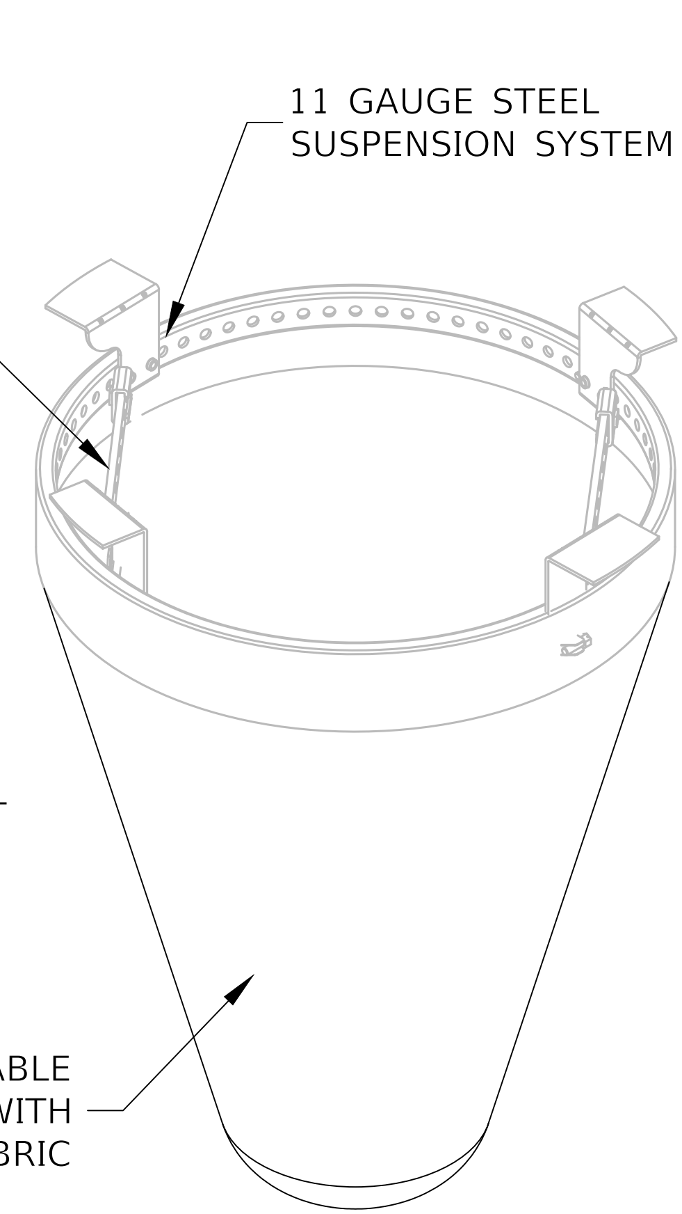
TYPICAL ROUND INLET FILTER
