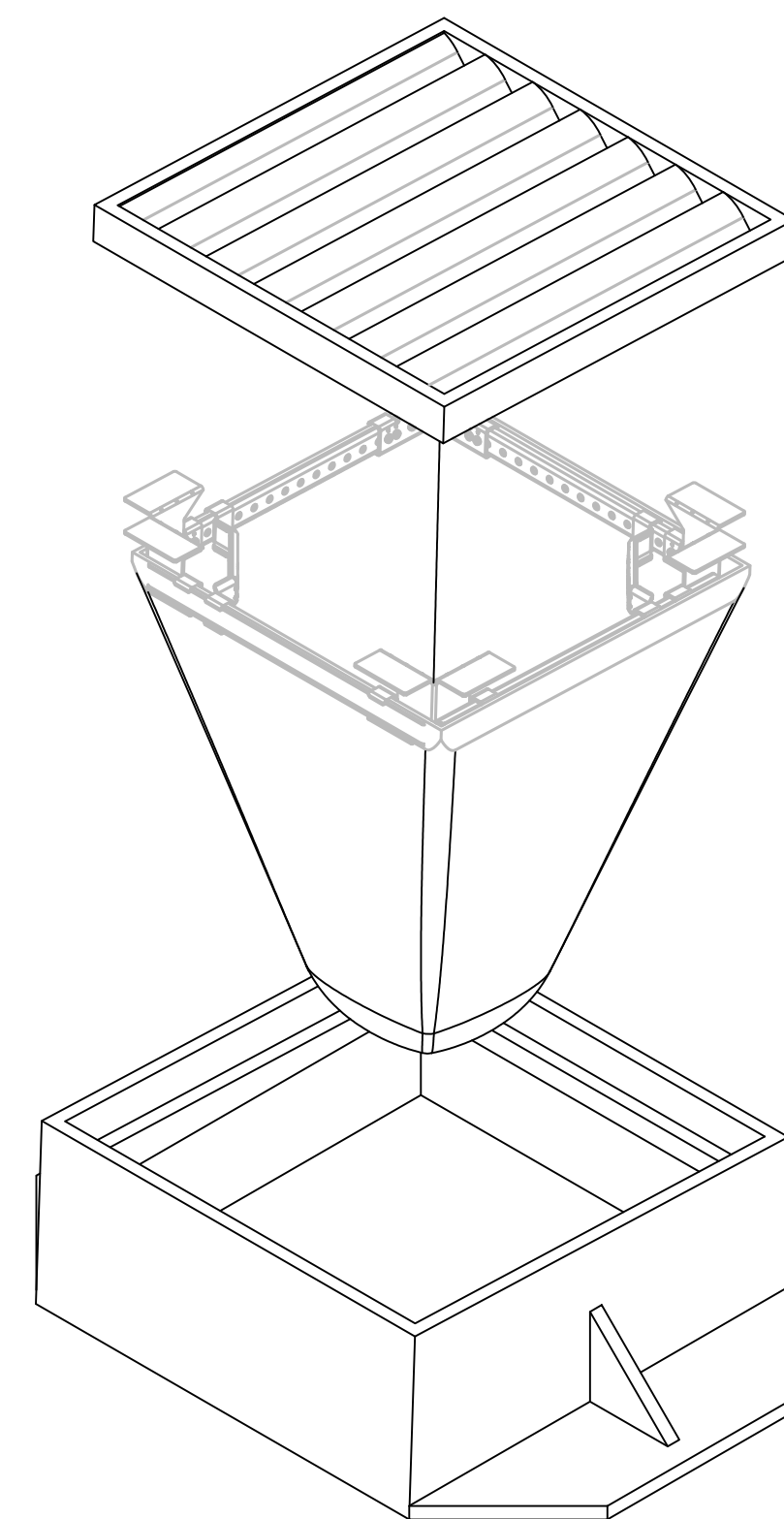
TYPICAL FLAT/RECTANGULAR/ROLLED CURB INLET FILTER
